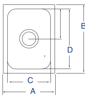
Top View - 10101-1
