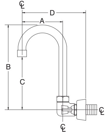
Gooseneck Faucet
