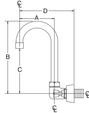
Gooseneck Faucet
