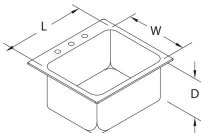
Inside Sink Bowl Dimensions
