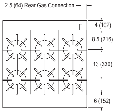
TOP VIEW - 12" OPEN TOP BURNERS
