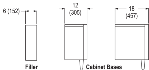
FRONT VIEWS
