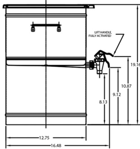
TDO-4 (Lift handle)
