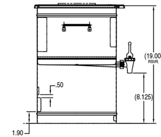
TDO-4 (Standard handle)
