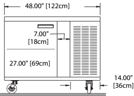
Elevation View 18648BUCM
