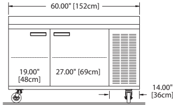
Elevation View 18660BSTM
