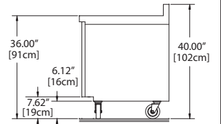
End View BSTM Models
