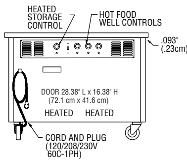
ELEVATION VIEW SH-3/SH-4/SH5/SH-6
