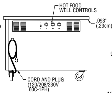
ELEVATION VIEW ALL SH-NU MODELS
