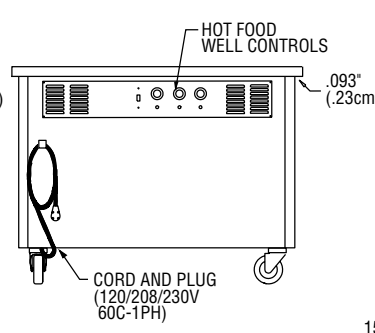
ELEVATION VIEW ALL SH-NU MODELS
