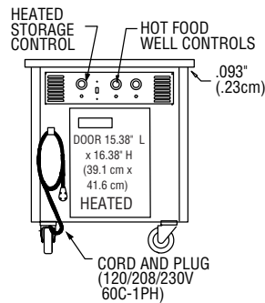
ELEVATION VIEW SH-2
