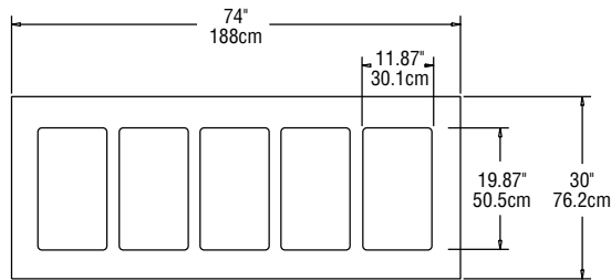
PLAN VIEW SH-5/SH-5-NU
