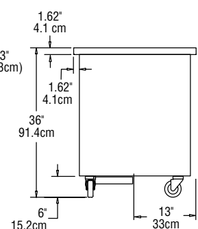
END VIEW ALL MODELS
