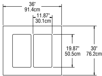
PLAN VIEW SH-2/SH-2-NU
