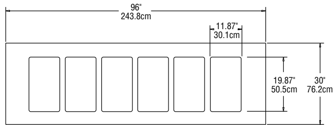
PLAN VIEW SH-6/SH-6-NU
