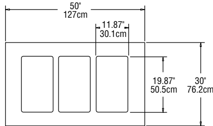
PLAN VIEW SH-3/SH-3-NU
