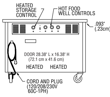
ELEVATION VIEW SH-3/SH-4/SH5/SH-6
