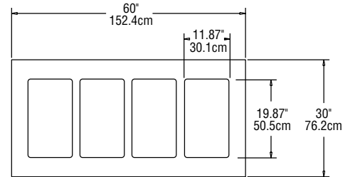
PLAN VIEW SH-4/SH-4-NU
