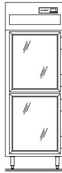
ELEVATION VIEW SSR1S-GH, SAR1S-GH, SMR1S-GH
