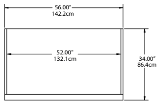
PLAN VIEW SSR2-S, SAR2-S, SMR2-S SSR2-SH, SAR2-SH, SMR2-SH
