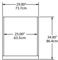
PLAN VIEW SSR1-S, SAR1-S, SMR1-S SSR1-SH, SAR1-SH, SMR1-SH
