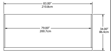
PLAN VIEW SSR3-S, SAR3-S, SMR3-S SSR3-SH, SAR3-SH, SMR3-SH
