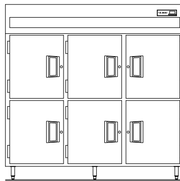
ELEVATION VIEW SSR3-SH, SAR3-SH, SMR3-SH
