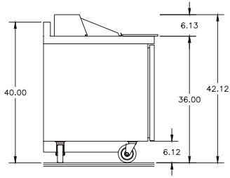
ST4460NP-8 Side View
