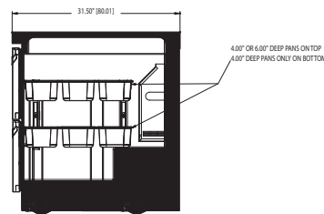
UCD4448N Right Side View
