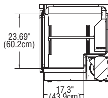
END VIEW UC4464N
