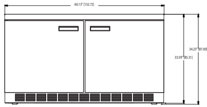
UC4560N Elevation View
