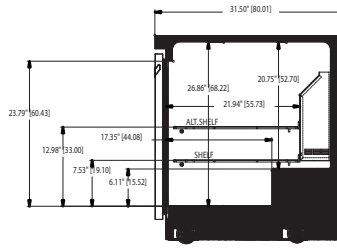
UC4560N Right Side View
