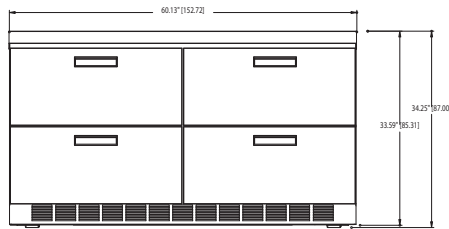
UCD4560N Elevation View
