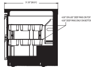
UCD4560N Right Side View
