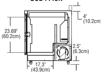
END VIEW STD4448N
