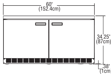
ELEVATION VIEW UC4460N
