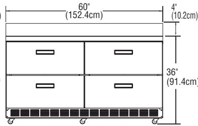
ELEVATION VIEW STD4460N
