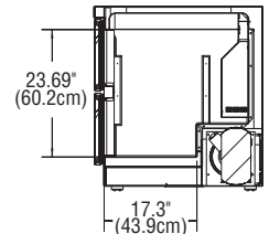
END VIEW UCD4460N
