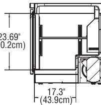
END VIEW UC4460N
