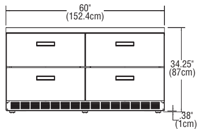
ELEVATION VIEW UCD4460N
