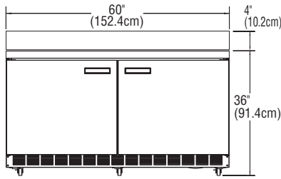
ELEVATION VIEW ST4460N
