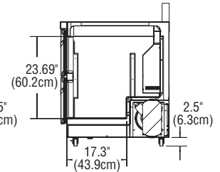
END VIEW STD4460N
