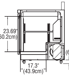
END VIEW ST4460N
