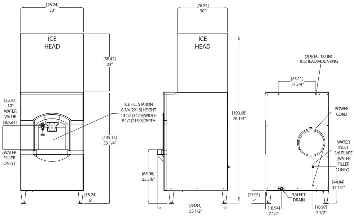
C0330 on HD30 hotel dispenser.
