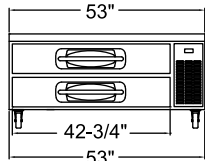
MBCB53 ELEVATION VIEW
