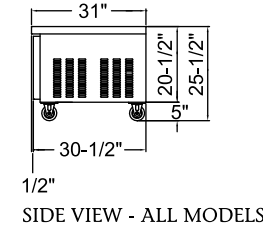
SIDE VIEW - ALL MODELS
