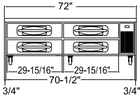
MBCB72 ELEVATION VIEW
