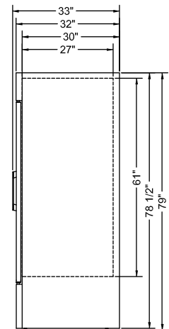
MBGR70H SIDE VIEW
