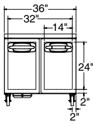
MBUR36A ELEVATION VIEW
