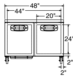
MBUR/MBUF48A ELEVATION VIEW
