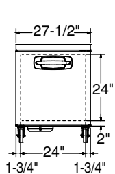
MBUR/MBUF27A ELEVATION VIEW
