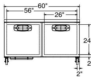
MBUR/MBUF60A ELEVATION VIEW
