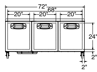
MBUR72A ELEVATION VIEW
