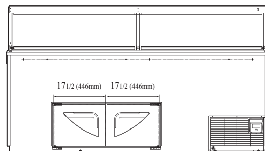
BACK VIEW
