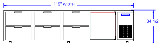
FRONT VIEW UCRD119A-6
