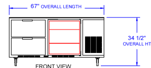
FRONT VIEW UCRD67A-2
