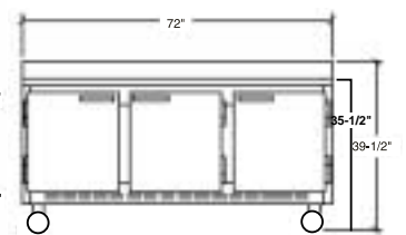
WTR72 Front
