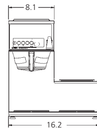
B-3WR Front View
