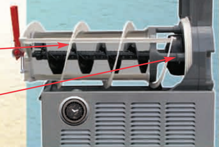
Cut-Away View
