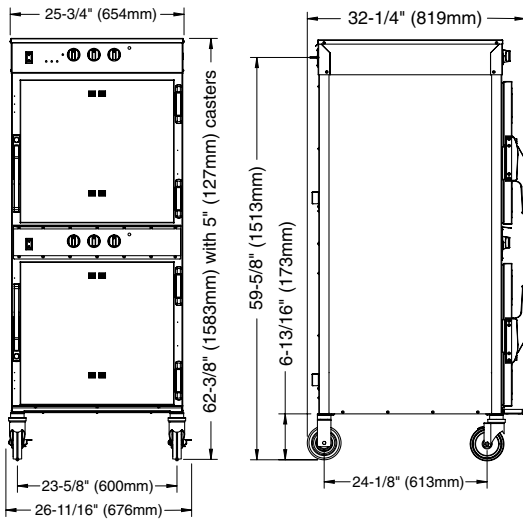
*60-11/16" (1540mm) - with optional 3-1/2" (89mm) casters *62-1/8" (1577mm) - with optional 6" (152mm) legs
