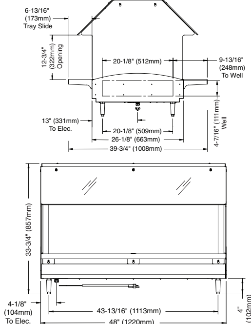
HFT2-300
