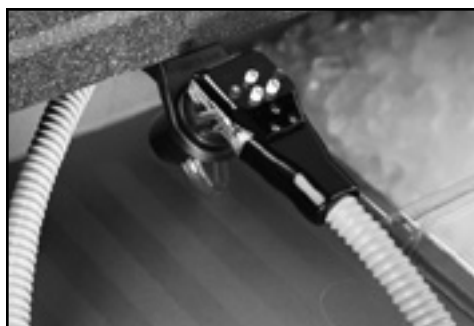
Premium quality 5-button, pre-mix soda gun by Wunder-Bar®. (shown on Cambar650DS model)
