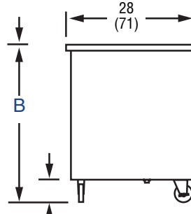
End View
