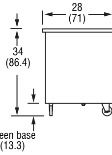
End View
