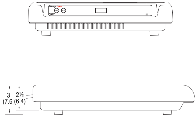
Unit shown with ½" (1.27 cm) feet.
