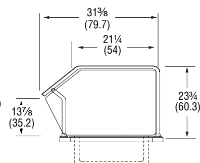
Single-Sided Buffet with Top Shelf - NSF
