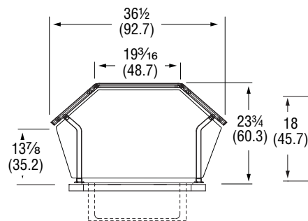
Double-Sided Buffet NSF
