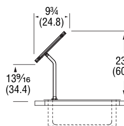
Single Sided Buffet Standard
