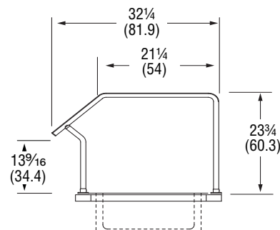
Single-Sided Buffet with Top Shelf - Standard
