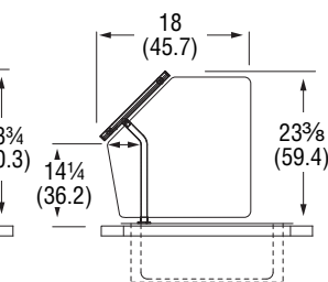
Single Sided Buffet NSF
