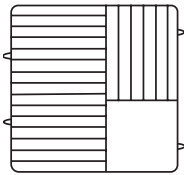
Plate Rack w/4 Extenders No. PM2110-4 Plate - D8 3 / 4 to D9 3 / 16 Max. H1, Cap. 21 2 pcs./14# • 4.3 cu.ft.
