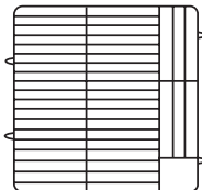
Plate Rack w/3 Extenders No. PM4407-3 Plate - D6 to D7 Max. H 3 / 4 , Cap. 44 2 pcs./11# • 4.2 cu.ft.
