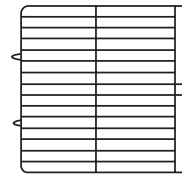
Plate Rack w/4 Extenders No. PM3208-4 Plate - D7 7 / 8 to D8 Max. H1, Cap. 32 2 pcs./12# • 4.3 cu.ft.
