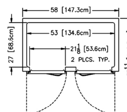
Plan - R/ACV232WUT
