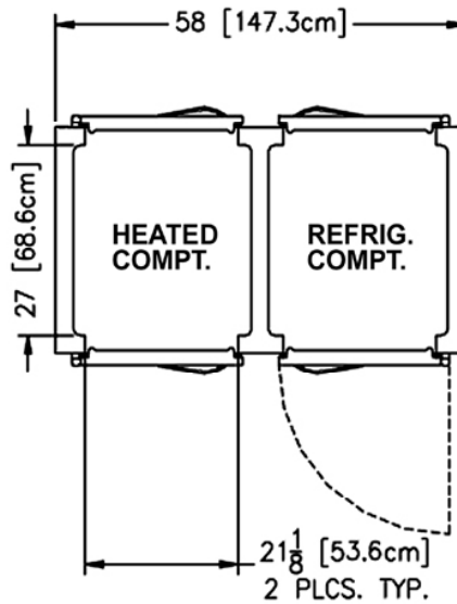
Plan - R/ADT232WPUT
