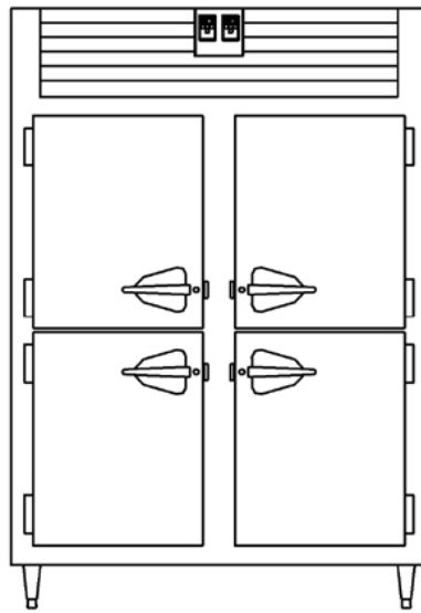
Elevation - R/ADH232WUT
