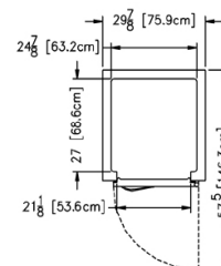
Plan - R/AHF132W
