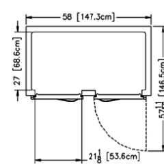
Plan - R/AHF232W
