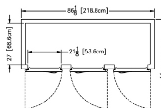
Plan - R/AHF332W
