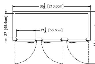
Plan - R/AHF332W
