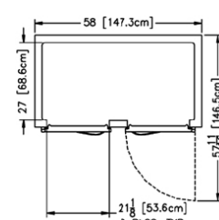
Plan - R/AHF232W
