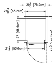
Plan - R/AHF132W
