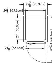
Plan - R/AHF132W
