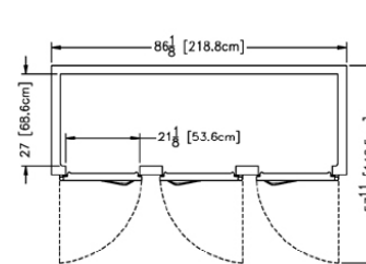
Plan - R/AHF332W
