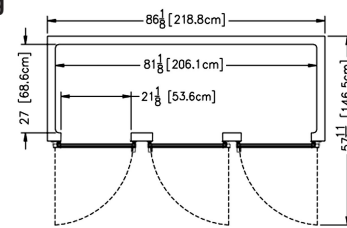
Plan - R/AHT132WUT
