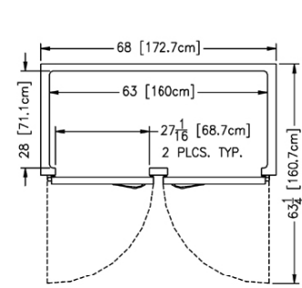
Plan - R/AIF232LUT
