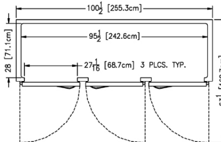
Plan - R/ARI332LUT
