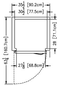
Plan - R/ARI132LUT
