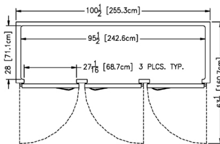
Plan - R/ARI332LUT
