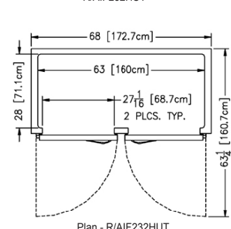
Plan - R/AIF232HUT
