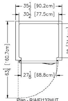
Plan - R/AIF132HUT
