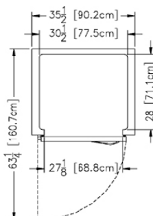
Plan - R/AIF132LUT
