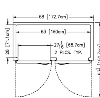
Plan - R/AIF232LUT
