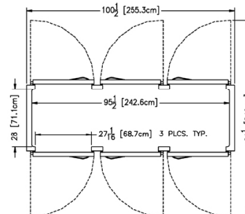
Plan - R/ARI132LPUT
