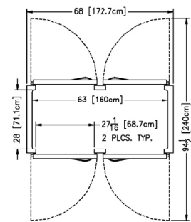
Plan - R/ARI232LPUT
