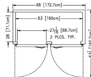
Plan - R/ARI232HUT
