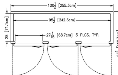
Plan - R/ARI332HUT
