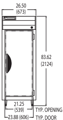
VF-1 FRONT VIEW
