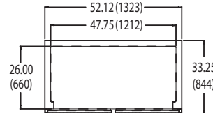
VF-2 TOP VIEW
