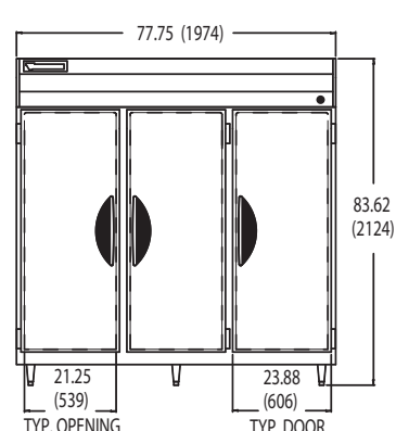
VF-3 FRONT VIEW
