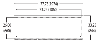
VF-3 TOP VIEW
