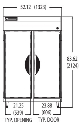
VF-2 FRONT VIEW
